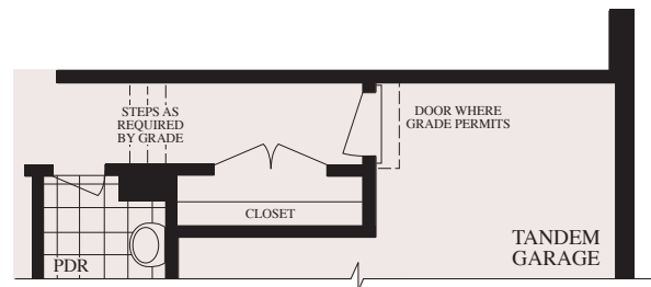
MAIN FLOOR PARTIAL PLAN IF LAUNDRY ON SECOND FLOOR
