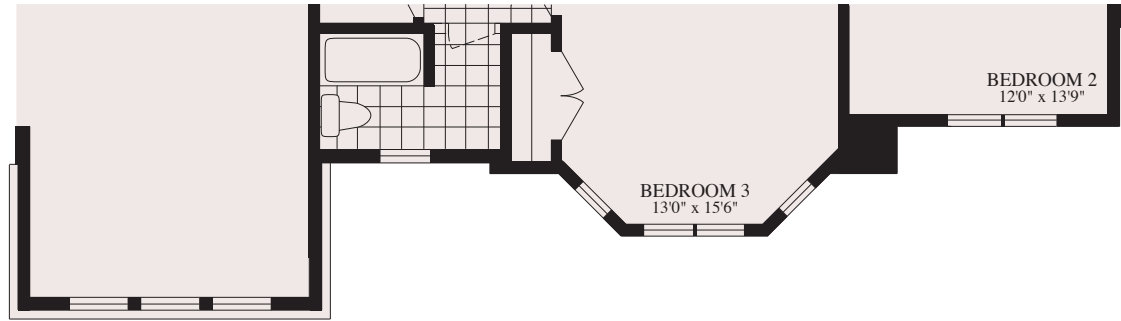
SECOND FLOOR OPTIONAL 4 BEDROOM OPEN TO BELOW ELEVATION C
