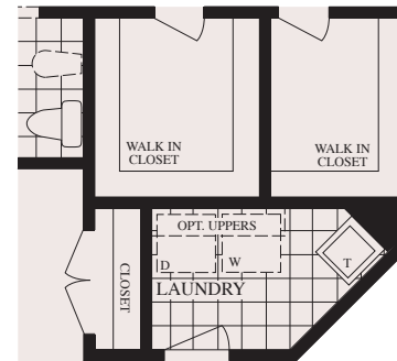
SECOND FLOOR PARTIAL PLAN 4 BEDROOM WITH FLEX SPACE WITH OPTIONAL LAUNDRY
