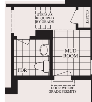
MAIN FLOOR PARTIAL PLAN IF LAUNDRY ON SECOND FLOOR
