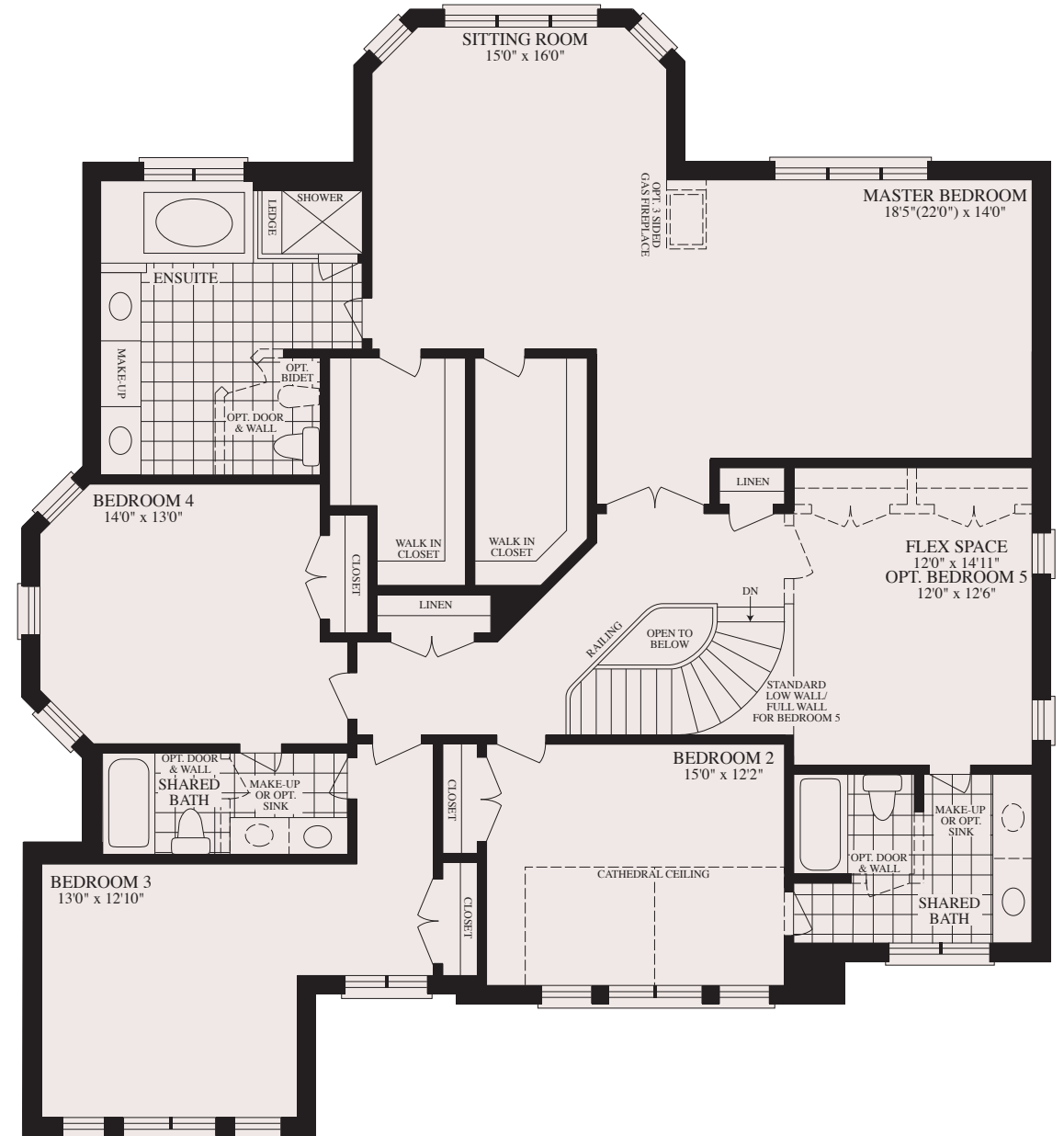
SECOND FLOOR 4 BEDROOM WITH FLEX SPACE ELEVATION A*
