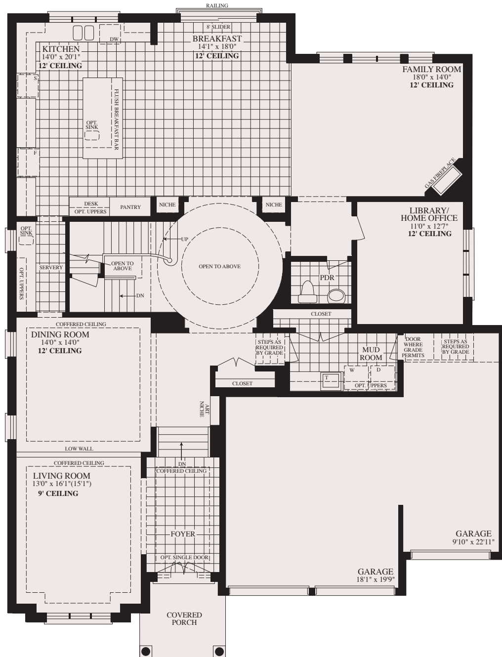
ENHANCED WALK-OUT MAIN FLOOR ELEVATION A*
